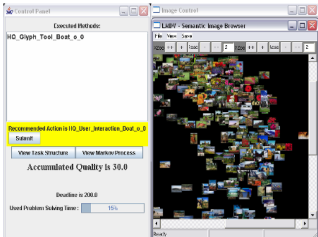
Figure 7: Screenshot of TIBOR in the midst of executing HQ_User_Interaction method: the control panel is on the left and the semantic image browser on the right.
