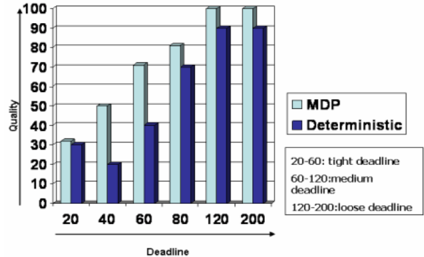
Figure 9: Comparison of Quality
