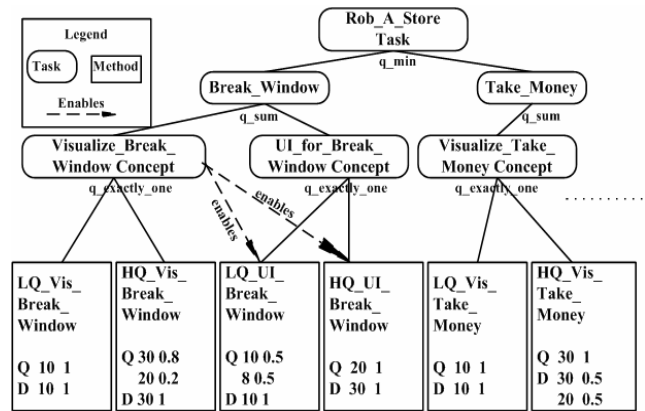
Figure 3: Taems Task Structure for Rob_A_Store Task
