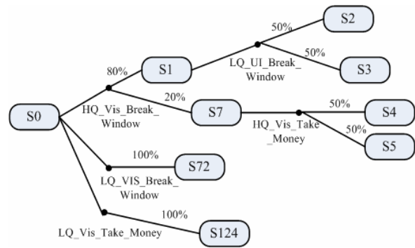
Figure 4: A partial view of the Markov Decision Process describing states, actions and transition probabilities for the Rob_A_Store task
